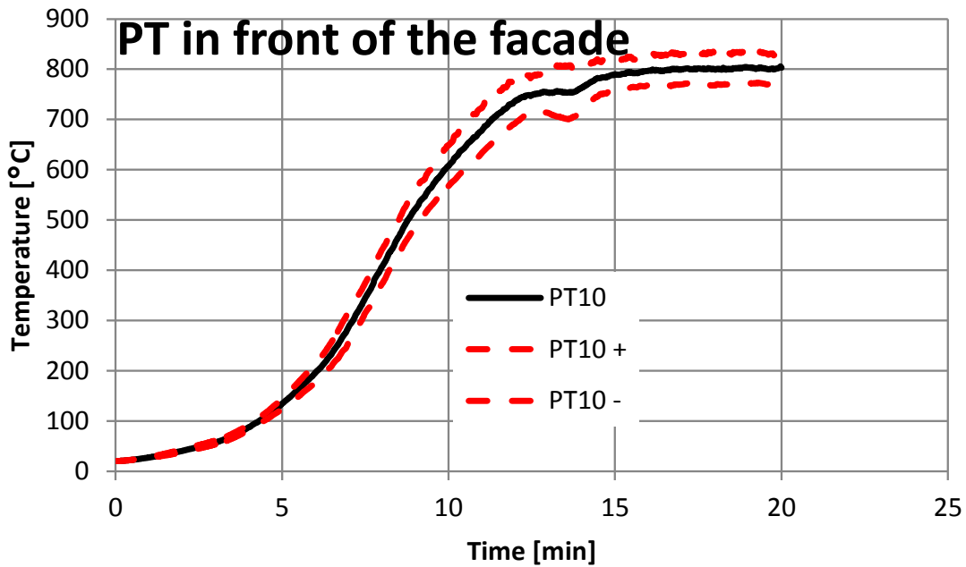
Figure 19. Temperature computed by the plate thermometer model in front of the ISO13785 - 2 façade. Here PT 10± refers to ± one standard deviation.
