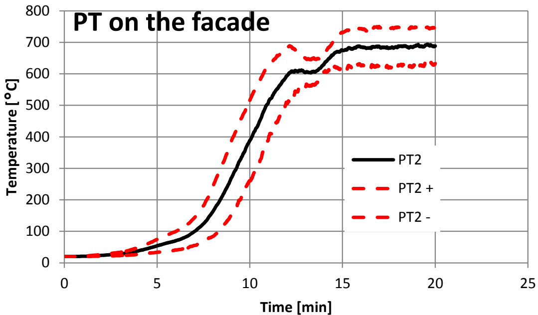
Figure 20. Temperature computed by the plate thermometer model on the ISO13785 - 2 façade. Here PT 2± refers to ± one standard deviation.
