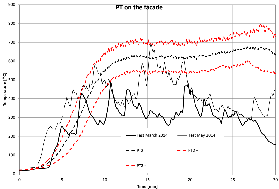
Figure 18. Temperature [°C] computed by the plate thermometer model on the BS 8414 - 1 façade. Here PT 2± refers to ± one standard deviation.
