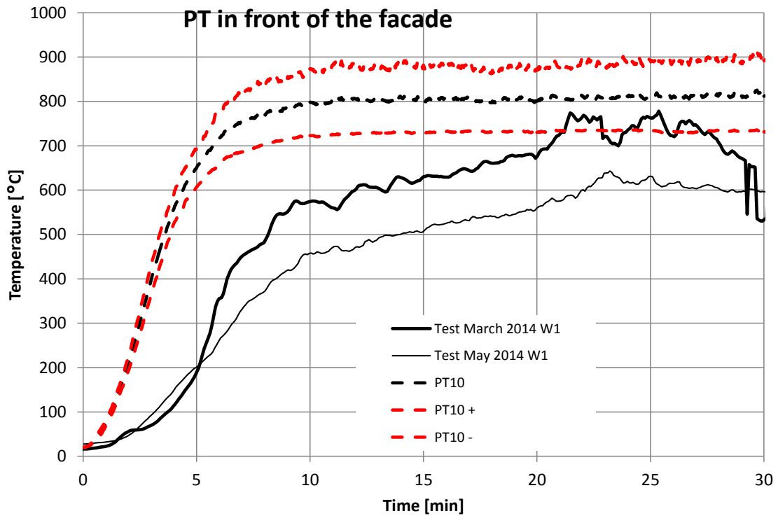
Figure 17. Temperature computed by the plate thermometer model in front of the BS 8414 - 1 façade, as indicated in Figure 7. Here PT 10± refers to ± one standard deviation.
